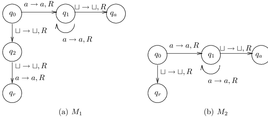
Figure 1: Two machines where L(M_1) = L(M_2) but \langle M_1 \rangle \notin TOUR_{TM} and \langle M_2 \rangle \in TOUR_{TM}
